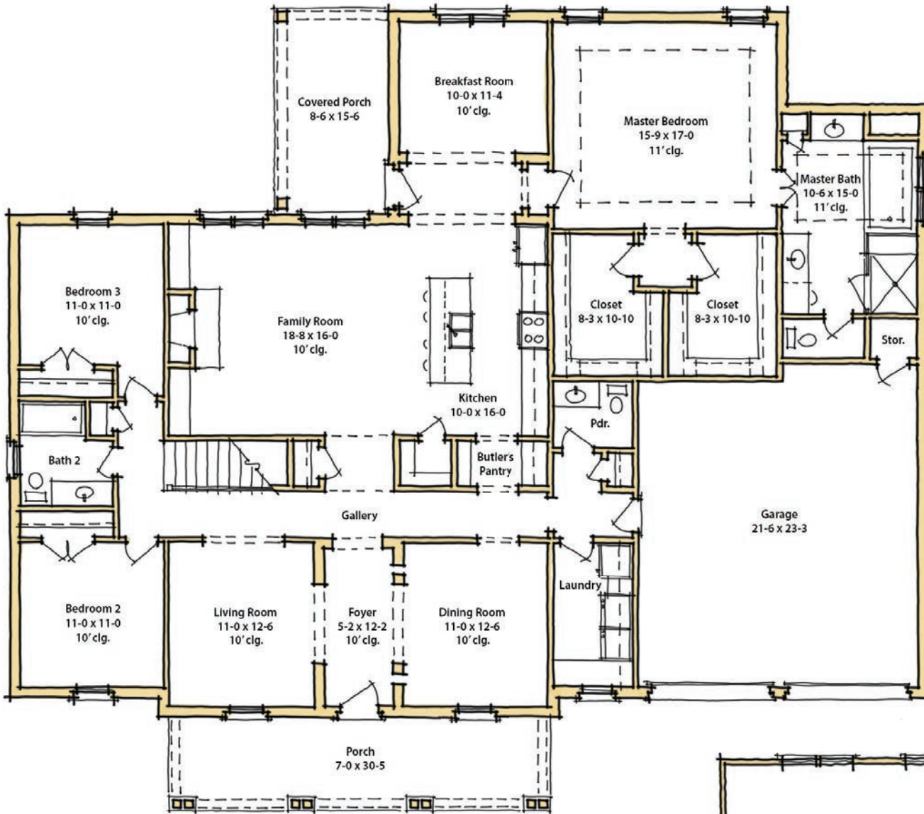
FIRST FLOOR
